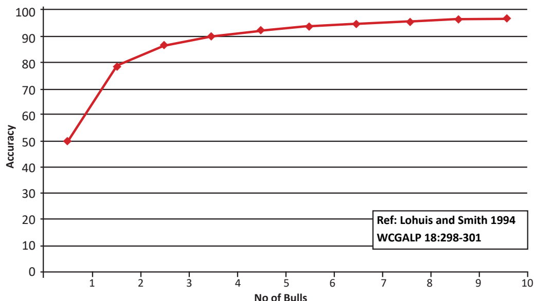
Figure 2. Accuracy of EBVs for a Bull Team when EBV Accuracy of Individuals is 50%. Note: as bulls within the team become related (eg. half sibs), the increase in accuracy decreases.
